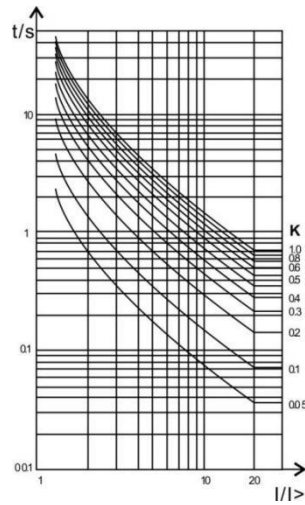
IDMT Very Inverse
