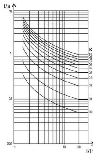
IDMT Extremely Inverse
