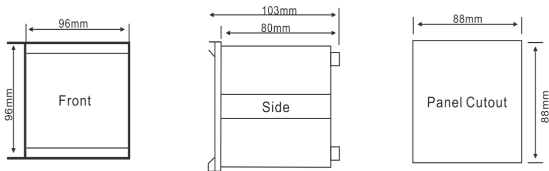
Figure3: Case Dimension
